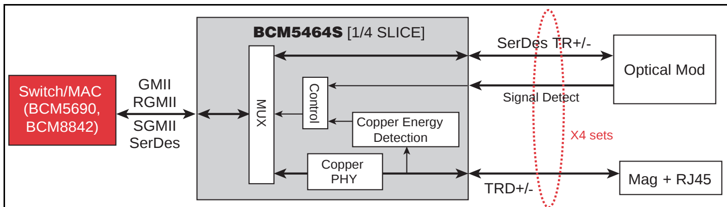
BCM5464S System Diagram
